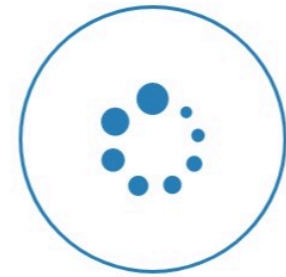
workflow management
